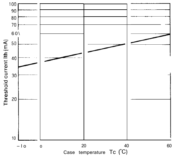
Fig. 69-3 Threshold Current vs. Temperature
