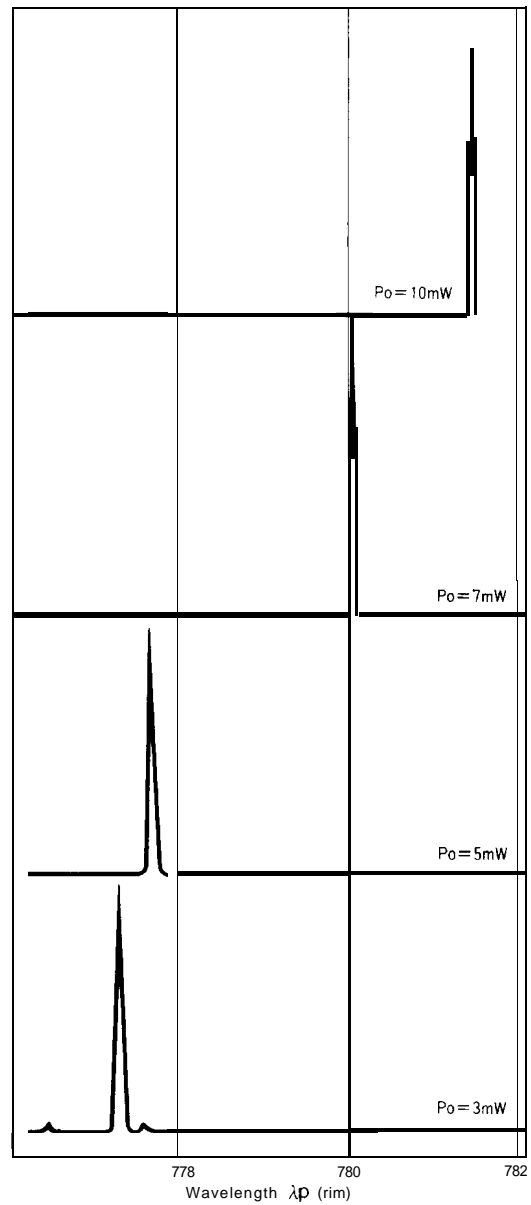
Fig. 69-5 Optical Power Output Dependence of Wavelength
