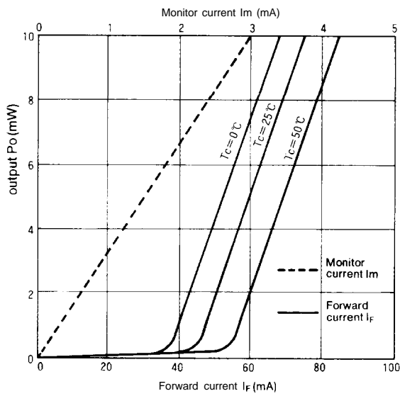
Fig. 69-3 Threshold Current vs. Temperature
